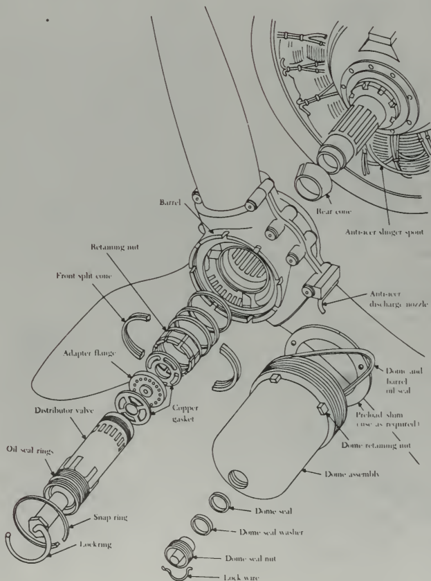
FIGURE 7-17. Typical hydromatic propeller installation.
